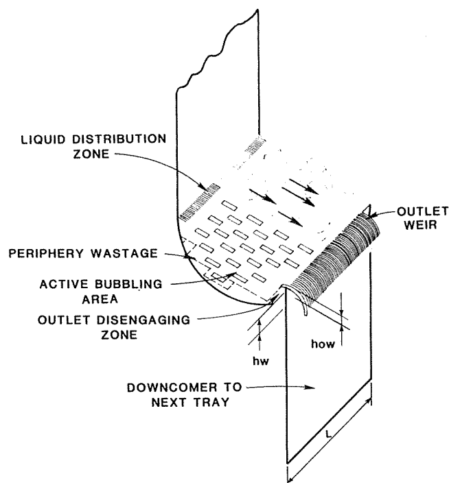
Figure 2. Typical contactor tray arrangement.
