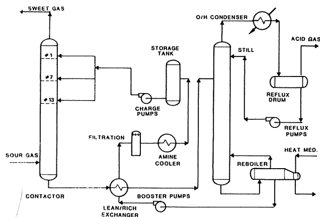
Figure 3. Process flow diagram for Forestburg Sweetening Plant.
