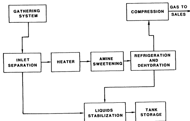
Figure 1. Block flow diagram for Forestburg Facility.
